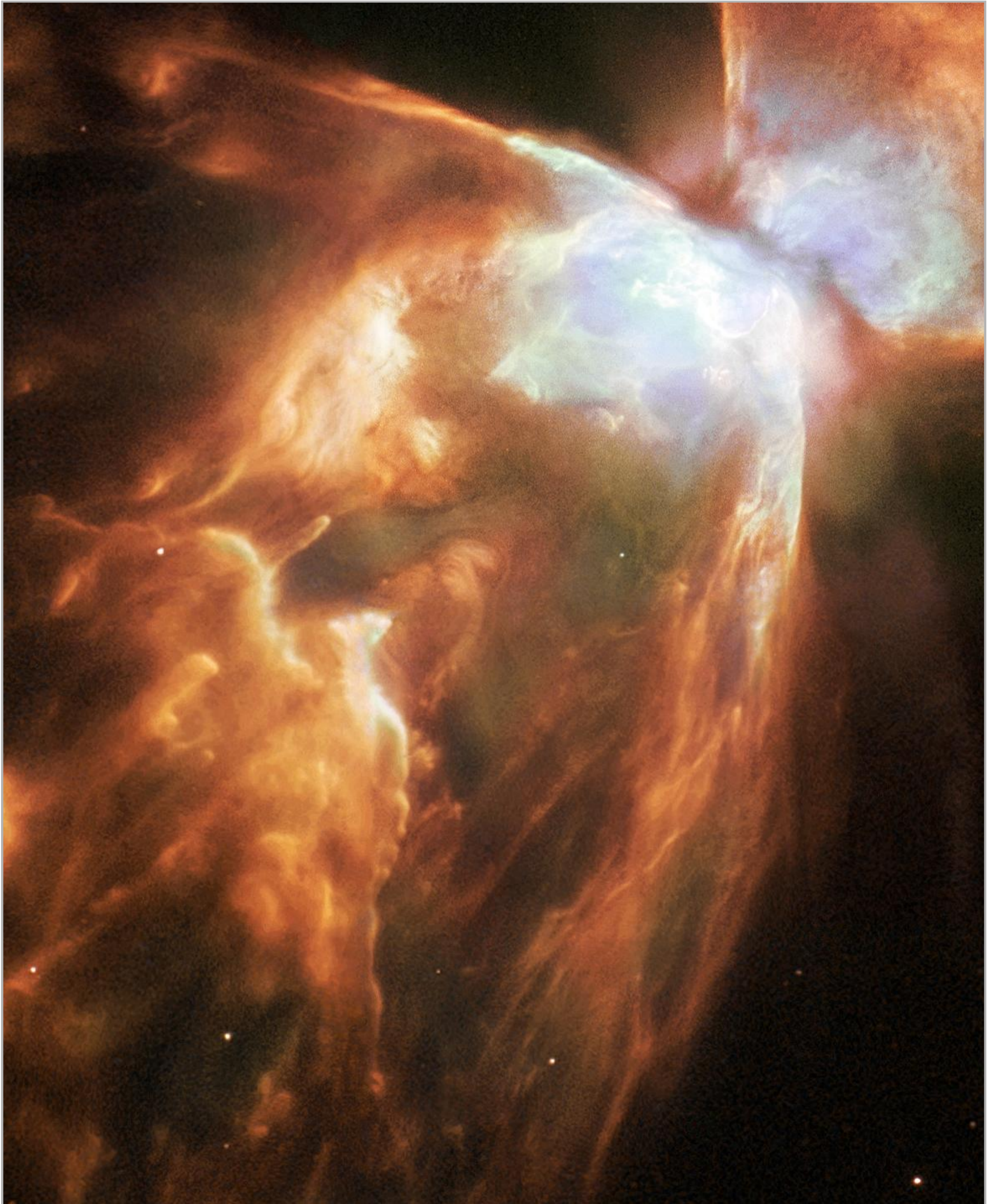
The Bug Nebula, NGC 6302, is one of the brightest and most extreme planetary nebulae known. At its centre lies a superhot, dying star smothered in a blanket of hailstones.
