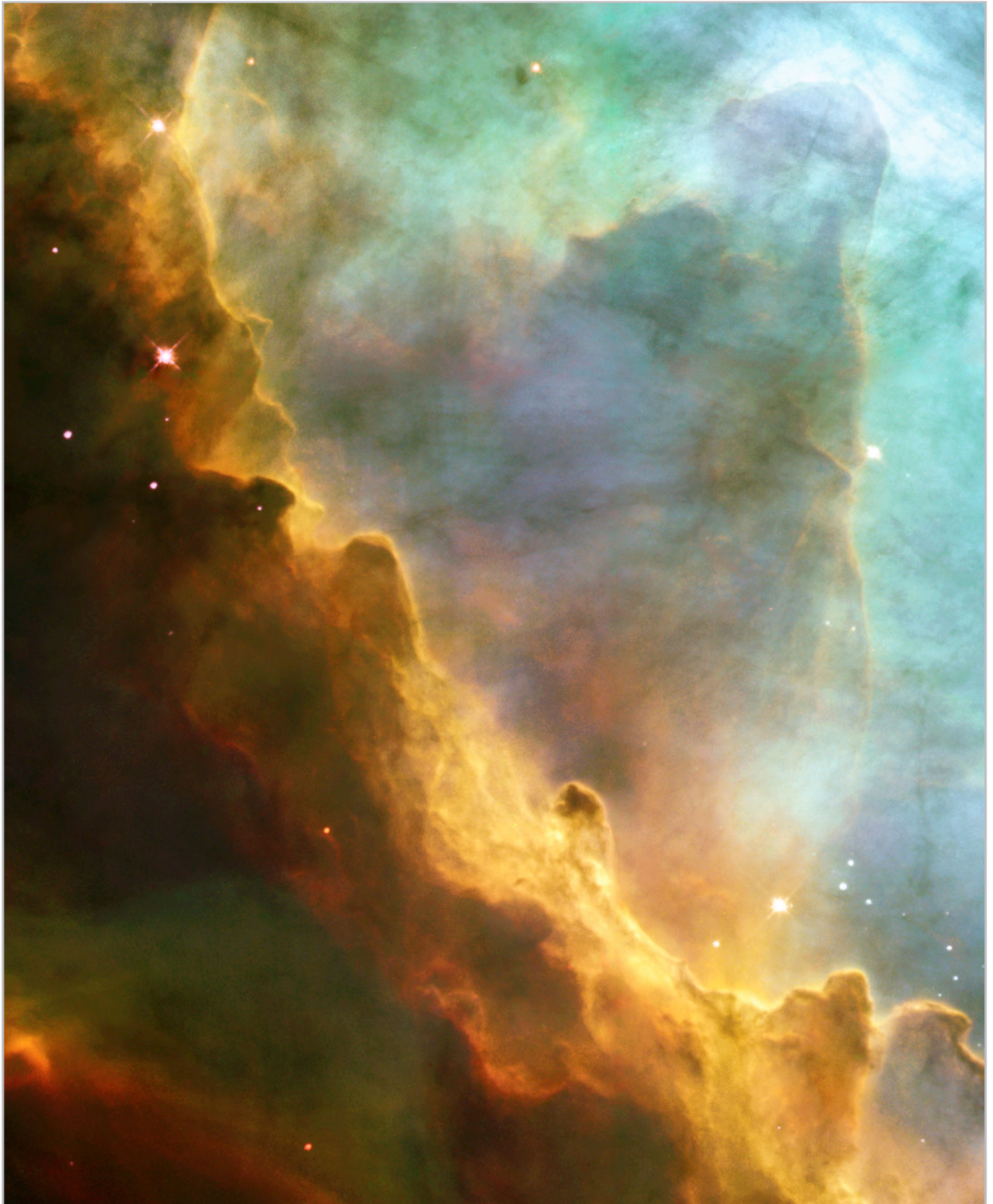
Like the fury of a raging sea, this image from the NASA/ESA Hubble Space Telescope shows a bubbly ocean of glowing hydrogen, oxygen, and sulphur gas in the extremely massive and luminous Omega Nebula. The wave-like patterns of gas have been sculpted and illuminated by young, massive stars.
